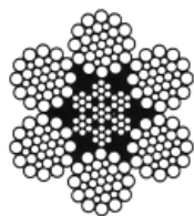
6 x 31 WARRINGTON SEALE WITH IWRC
