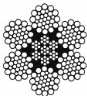
6 x 31 WARRINGTON SEAL WITH IWRC
