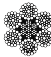
6 x 36 WARRINGTON SEALE WITH IWRC
