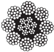
8 x 25 SPIN RESISTANT WITH IWRC
