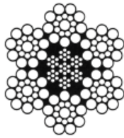
6 x 19 SEALE WITH IWRC
