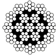
19 x 7 ROTATION RESISTANT WITH WIRE STRAND CORE
