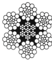
6 x 26 WARRINGTON SEALE WITH IWRC
